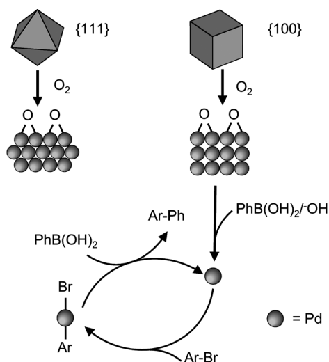
Figure 4. Mechanism of O 2 -promoted leaching on Pd NCs.
